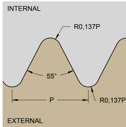
Whitworth (W)
