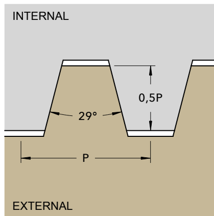
ACME
