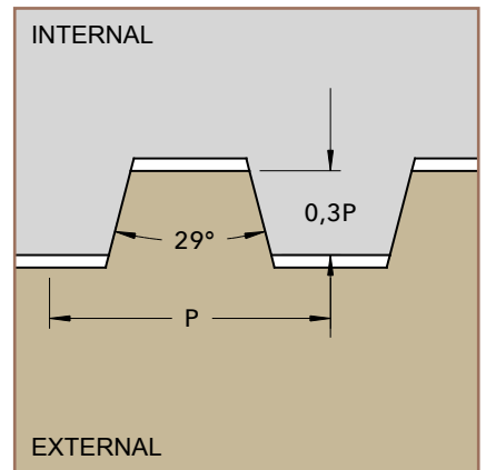
STUB ACME
