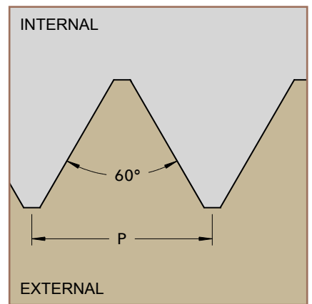
NPSF
