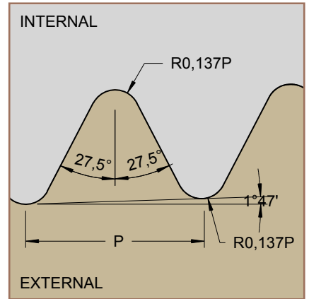
BSPT
